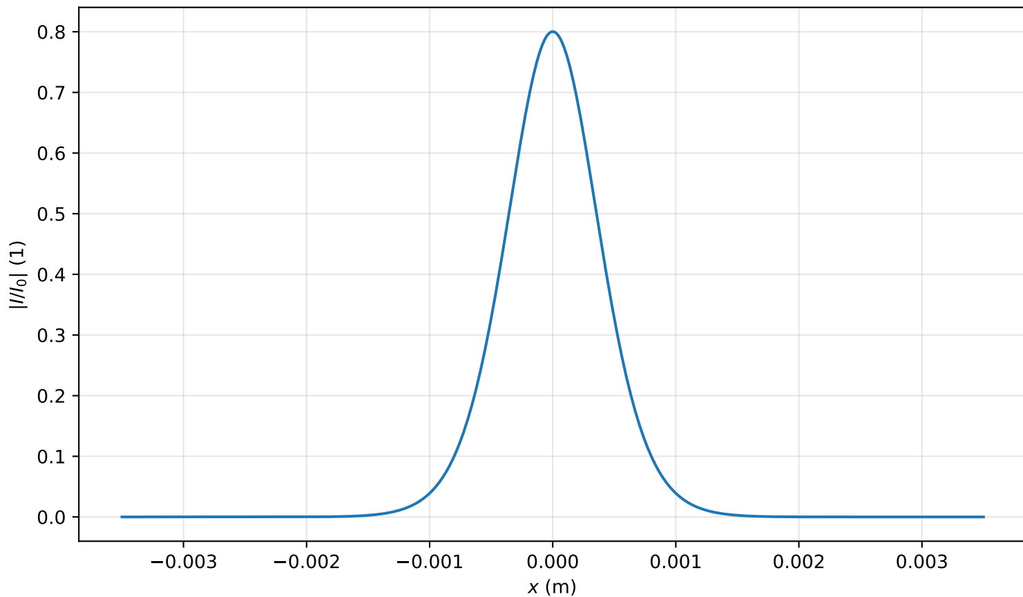
Intensity profile I(x, y = 0, z = 1.751m)/I_0 , P_{in}=0.4P_{cr} , artificial time
